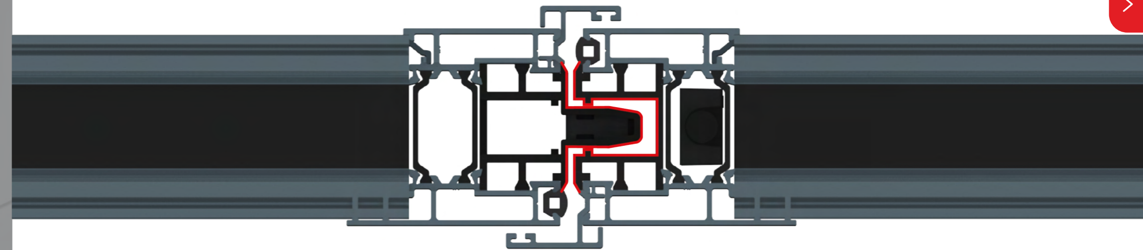
Pictured: New Wave Door Sliding Sashes Interlock Viewed From Above
